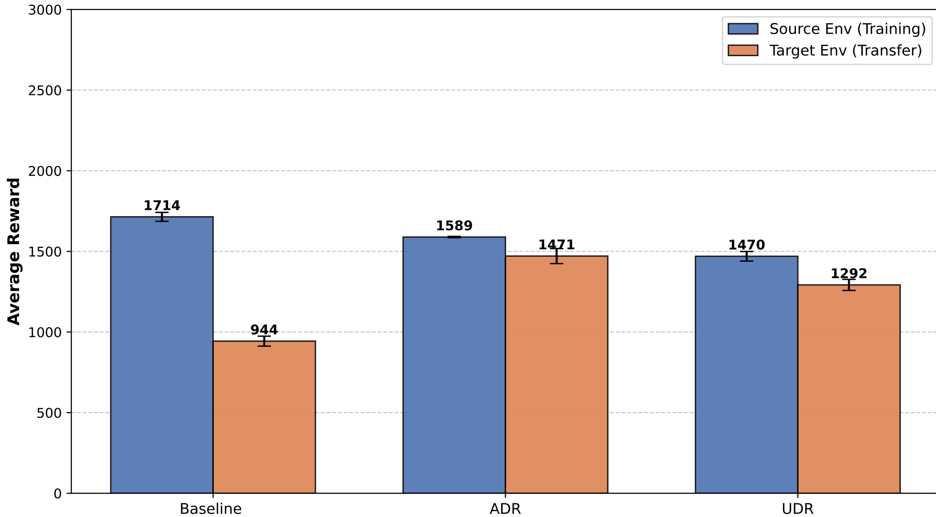
Robustness Comparison: Baseline vs ADR vs UDR
