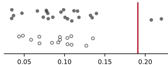
junction (bits)
