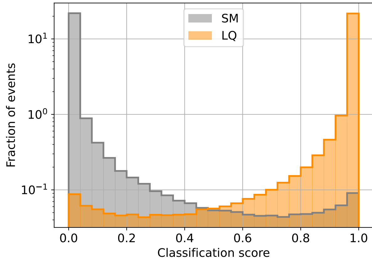
Model A - SM vs LQ
