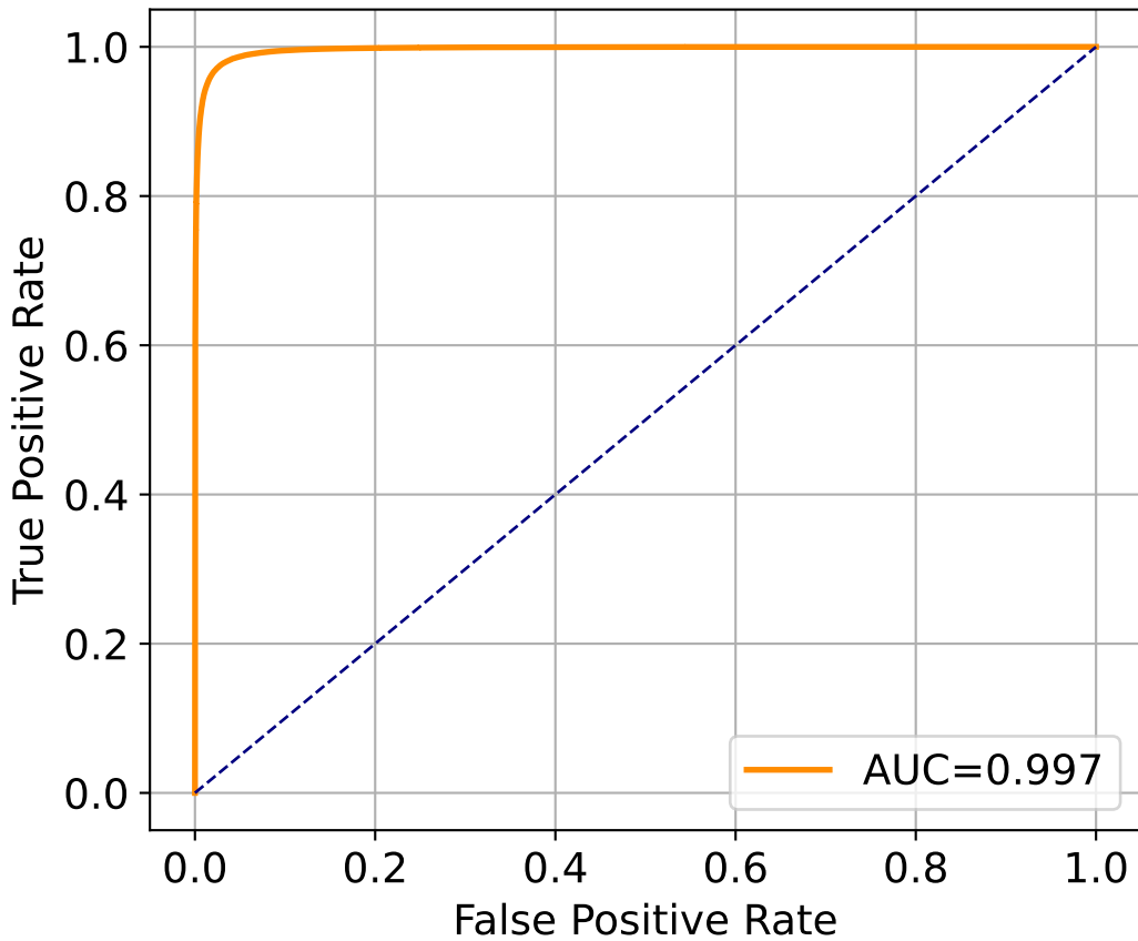
ROC Curve: SM vs LQ
