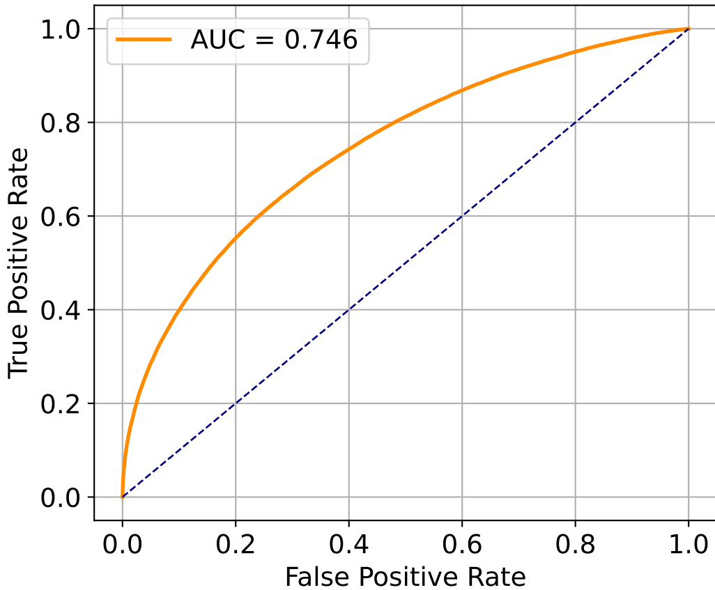
ROC Curve: SLQ vs VLQ
