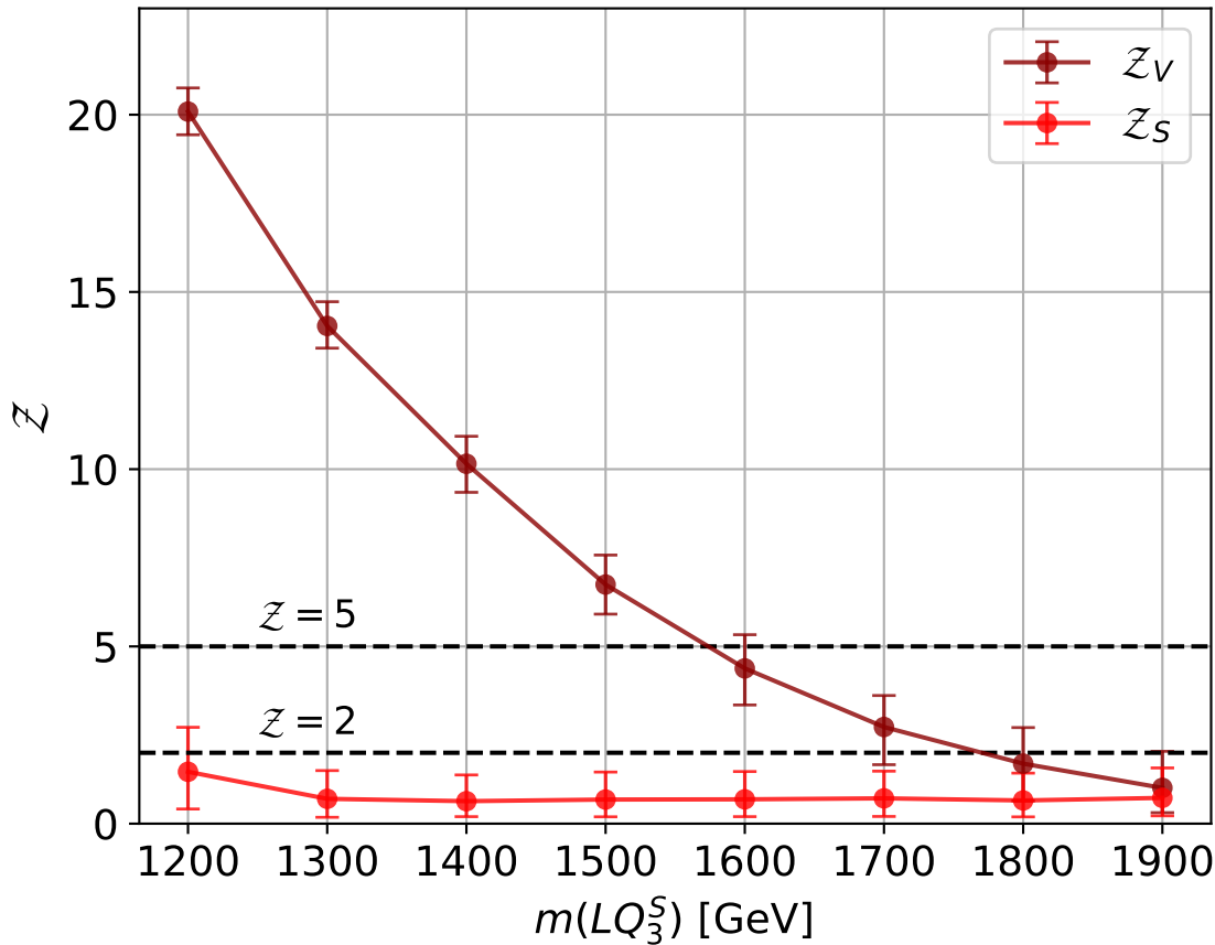
Pseudo-experiments build with SLQ
