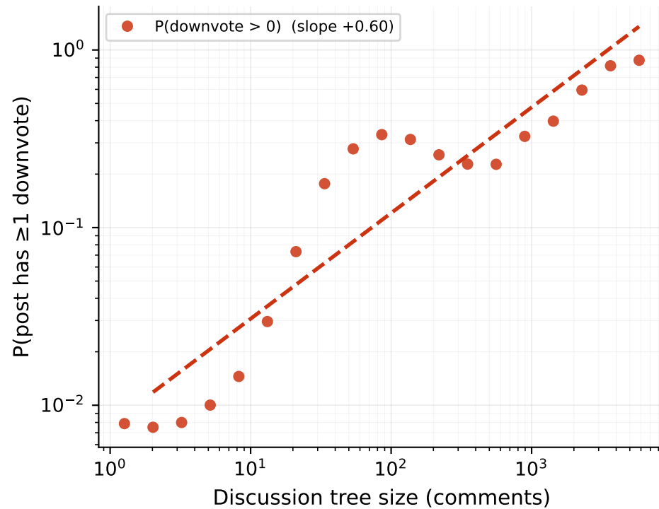
b (b) probability of being downvoted
