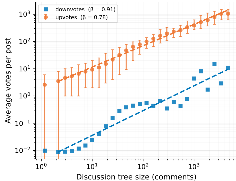
a (a) upvotes vs downvotes scaling
