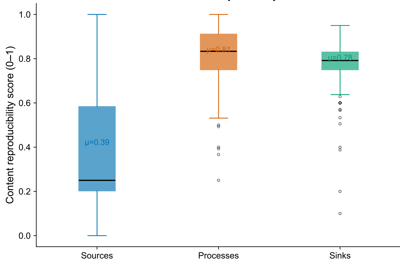
Content score by node layer
