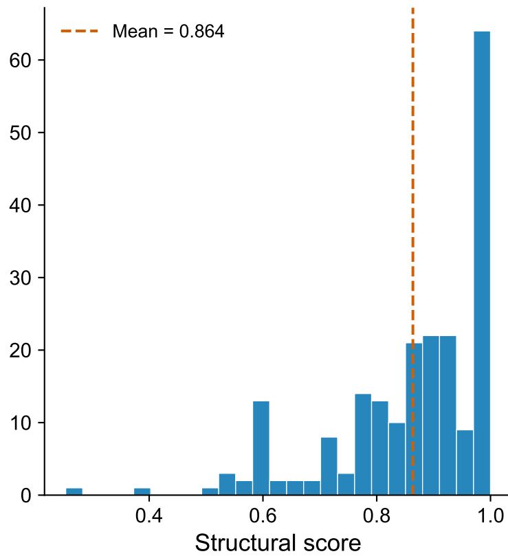
Score distributions — gemini-3.1-pro-preview, T = 0
