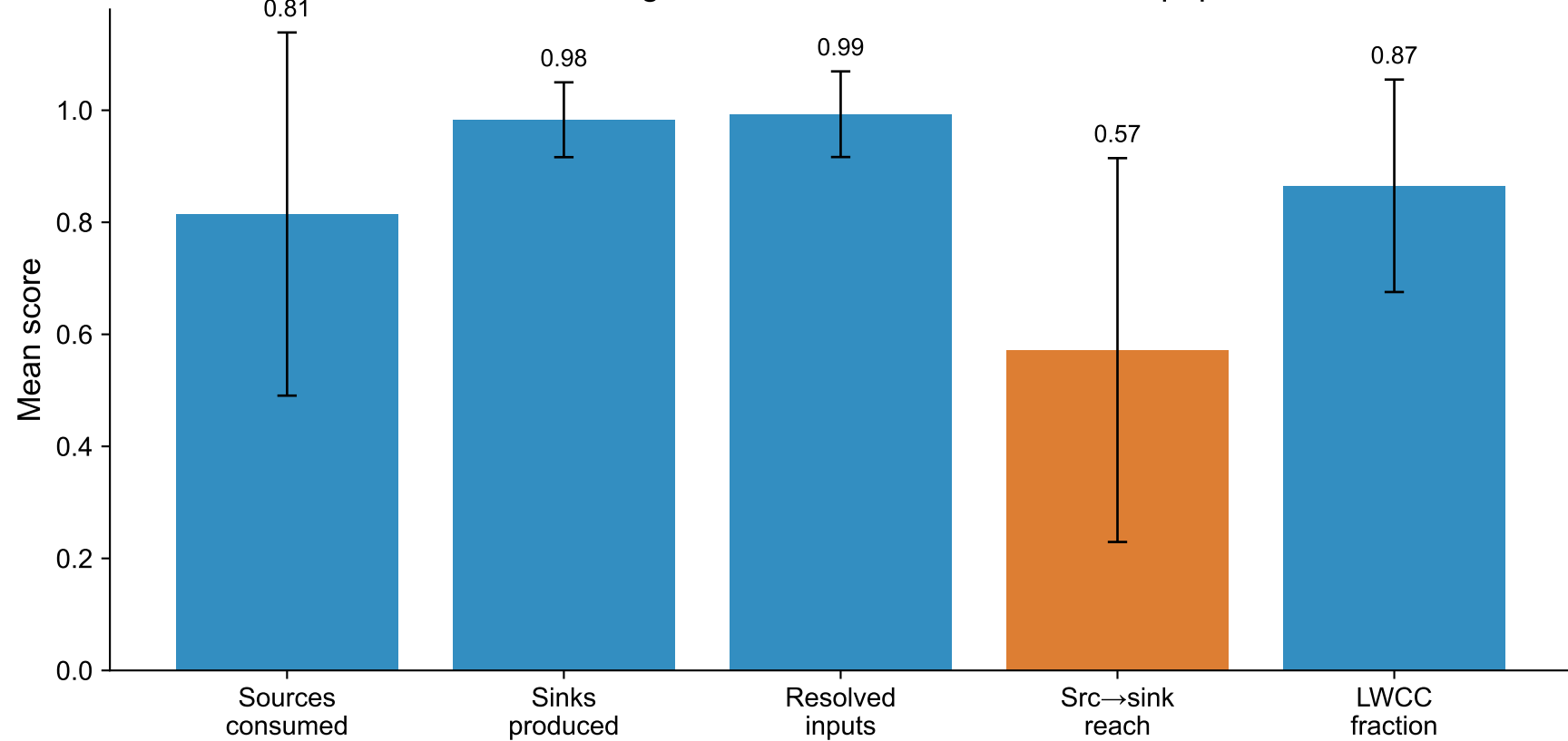
Structural wiring metrics — mean \pm std across all papers
