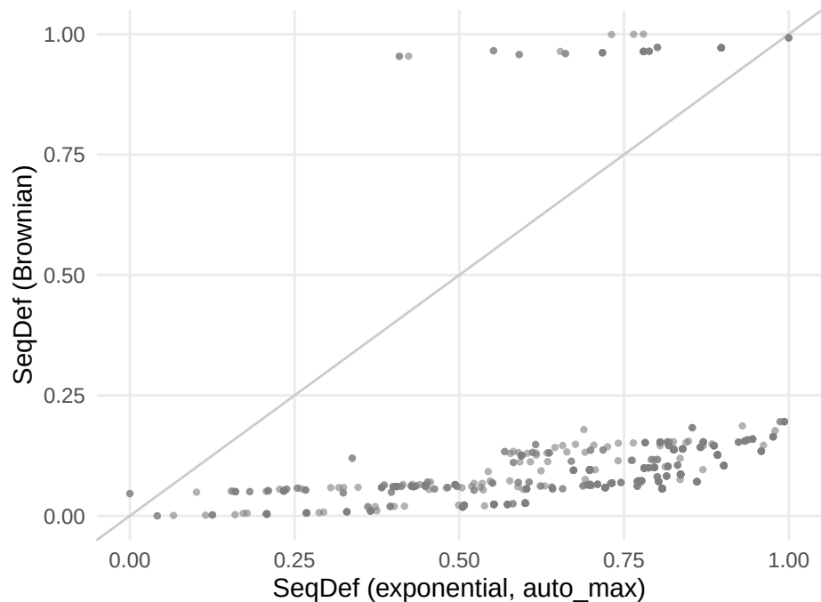
B Rankings differ (Spearman rho = 0.63)
