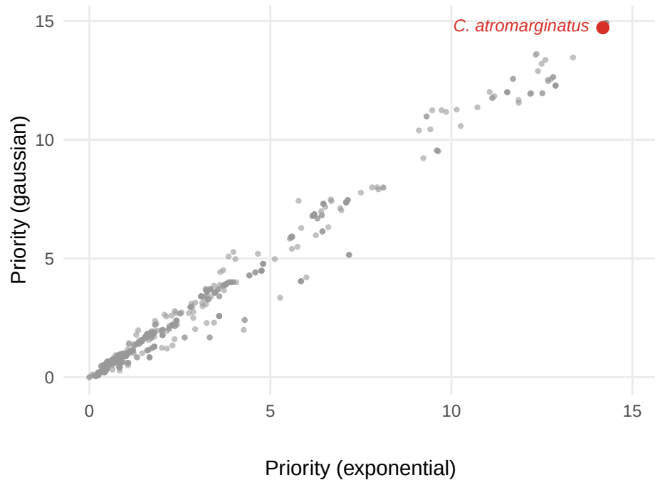
B MCC priority: exponential vs gaussian
