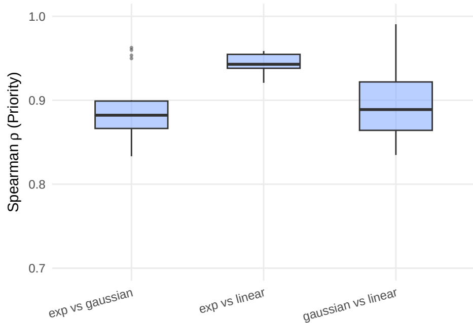
A Cross-kernel ranking agreement (posterior)
