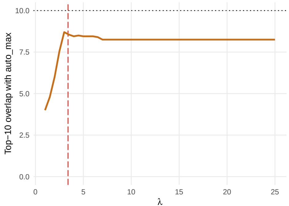
B Top-10 priority overlap across lambda
