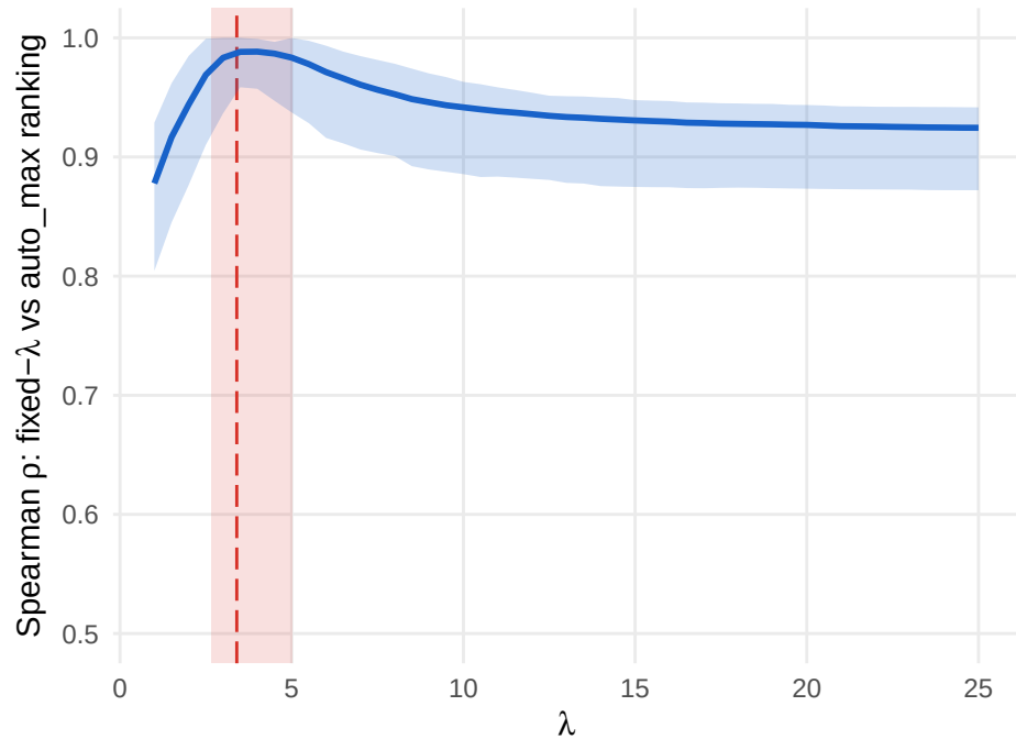
A Ranking stability across lambda (all 877 species)
