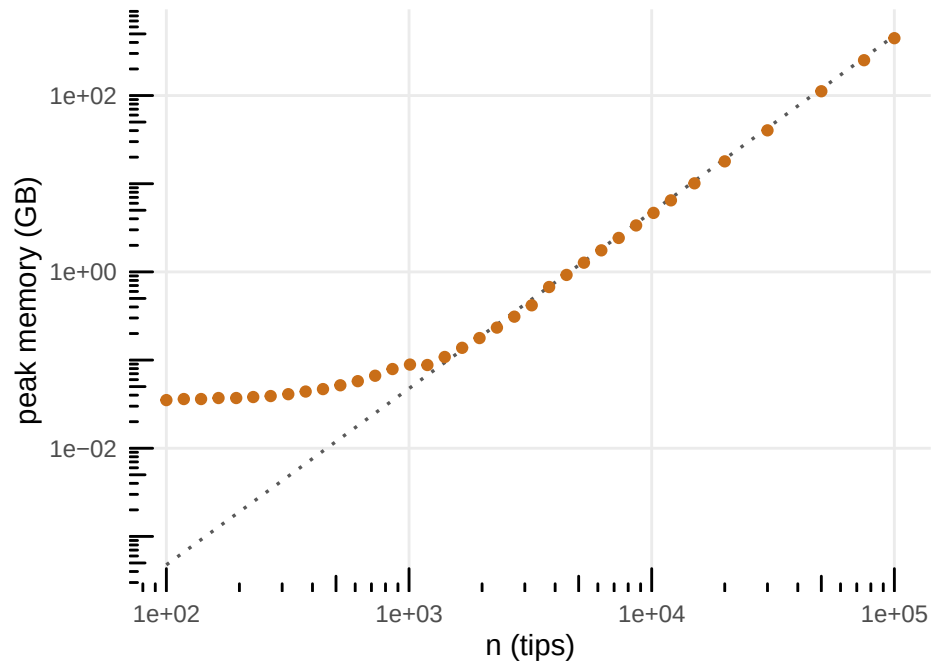
B Peak memory (dotted = O(n^2) )
