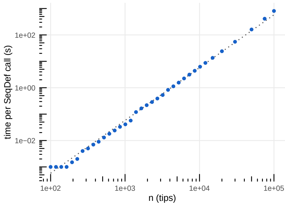
A Runtime, single \lambda (dotted = O(n^2) ; fitted slope 2.09)
