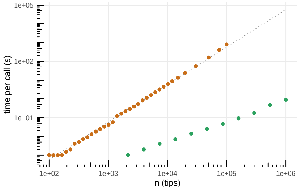
A Runtime: dense O(n^2) vs exponential traversal O(n)
