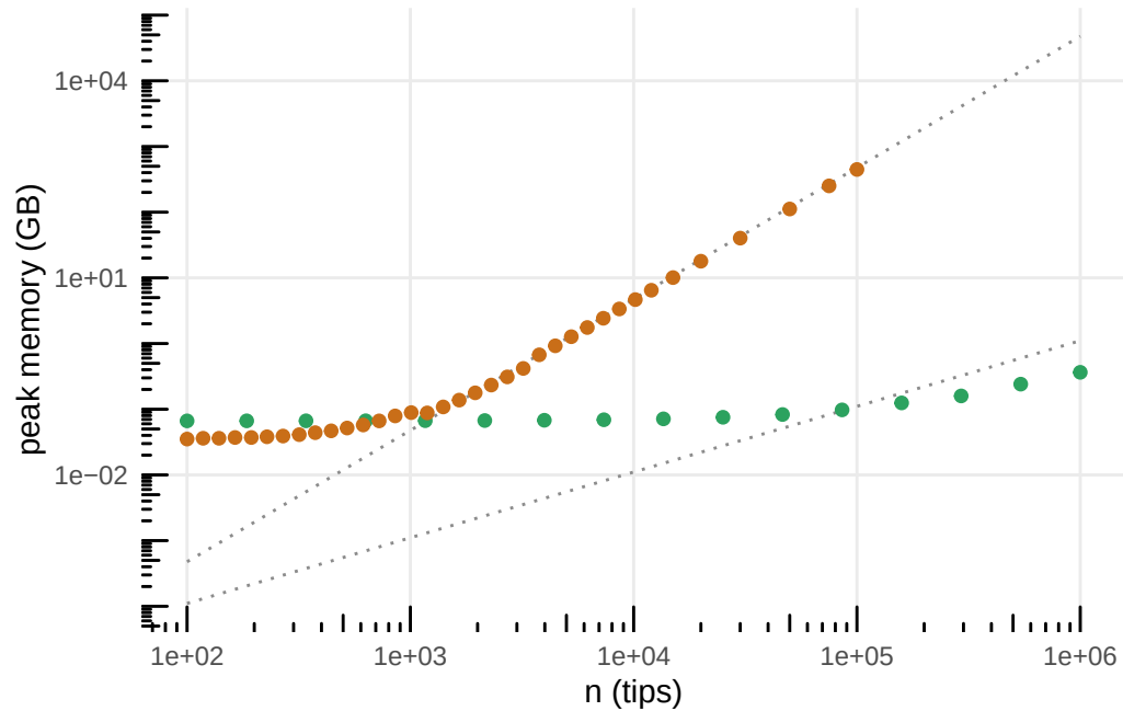
B Peak memory: dense O(n^2) vs traversal O(n)
