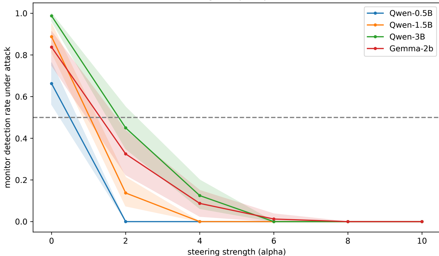
Minimal steering collapses probe detection
