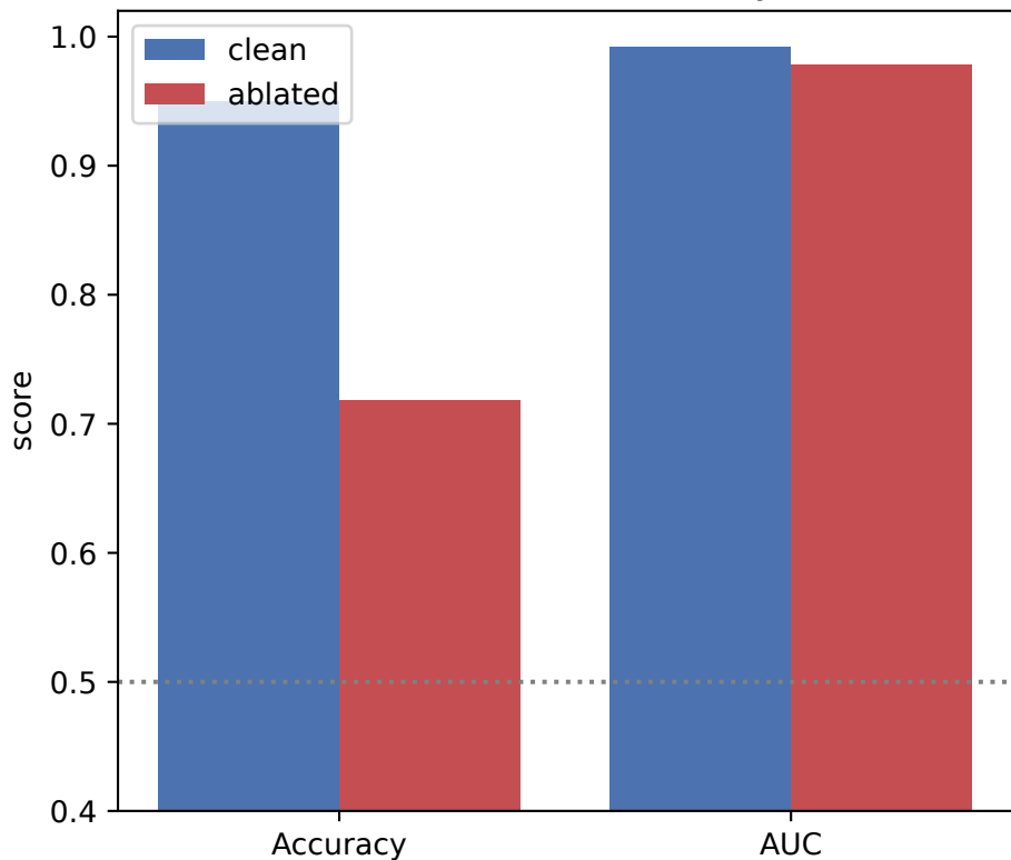
Qwen-3B critical-MLP ablation: accuracy falls, AUC intact
