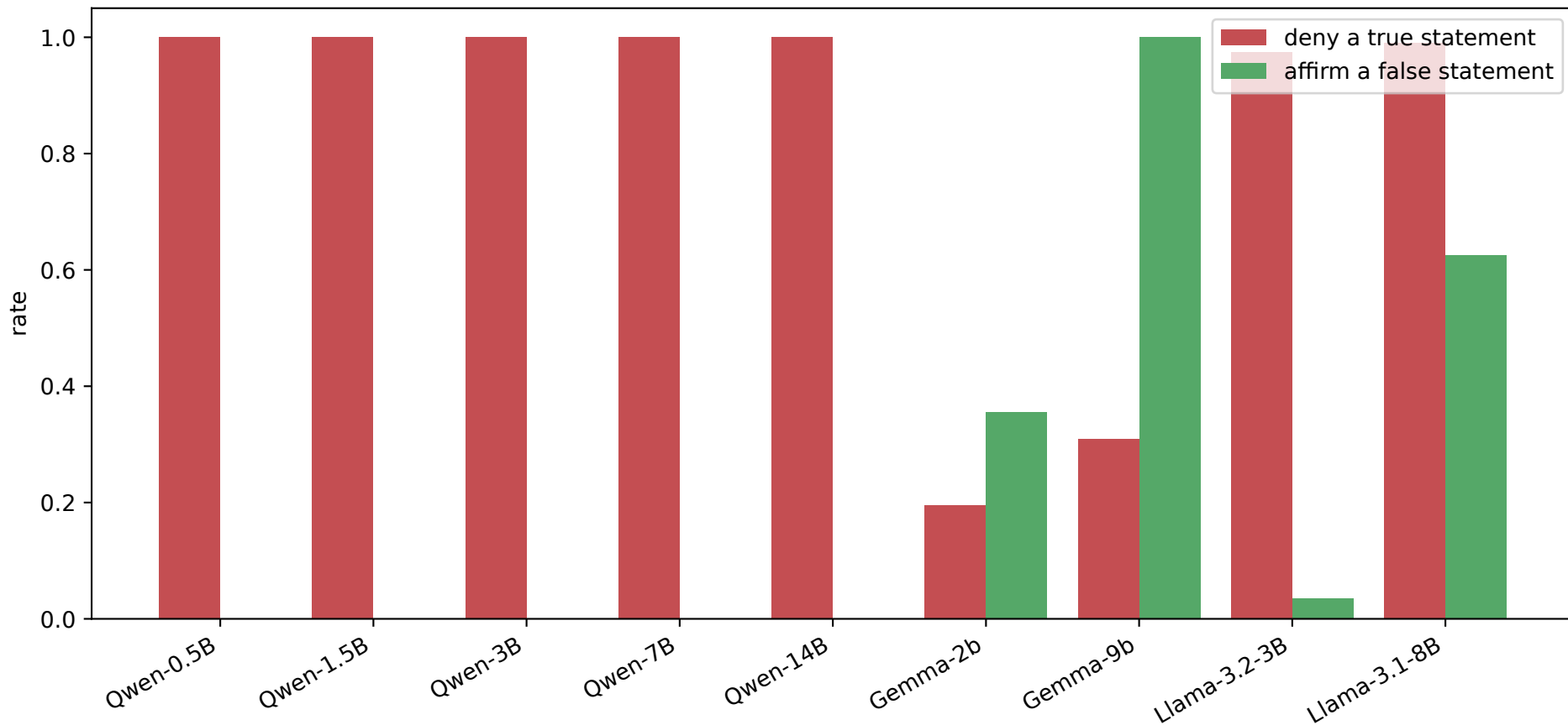
Denial bias: how each model lies
