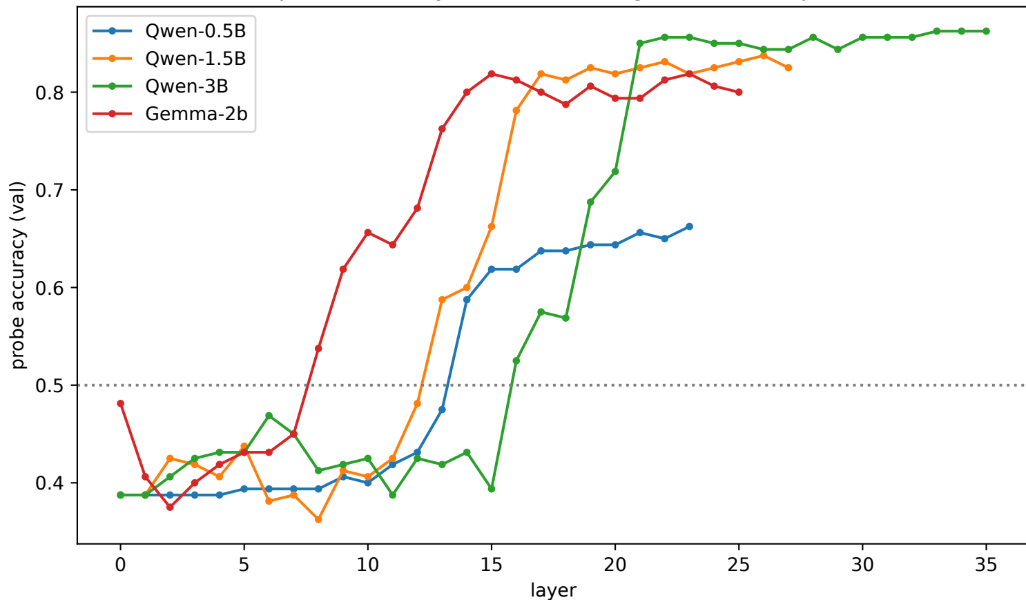
Deception is linearly decodable, rising to a mid-late plateau
