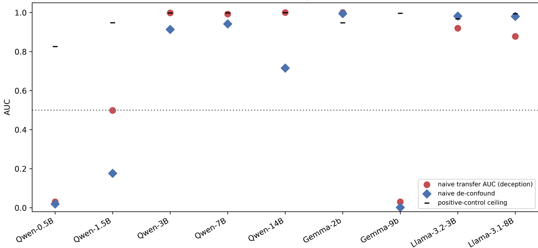
Nine models, nine uninterpretable verdicts
