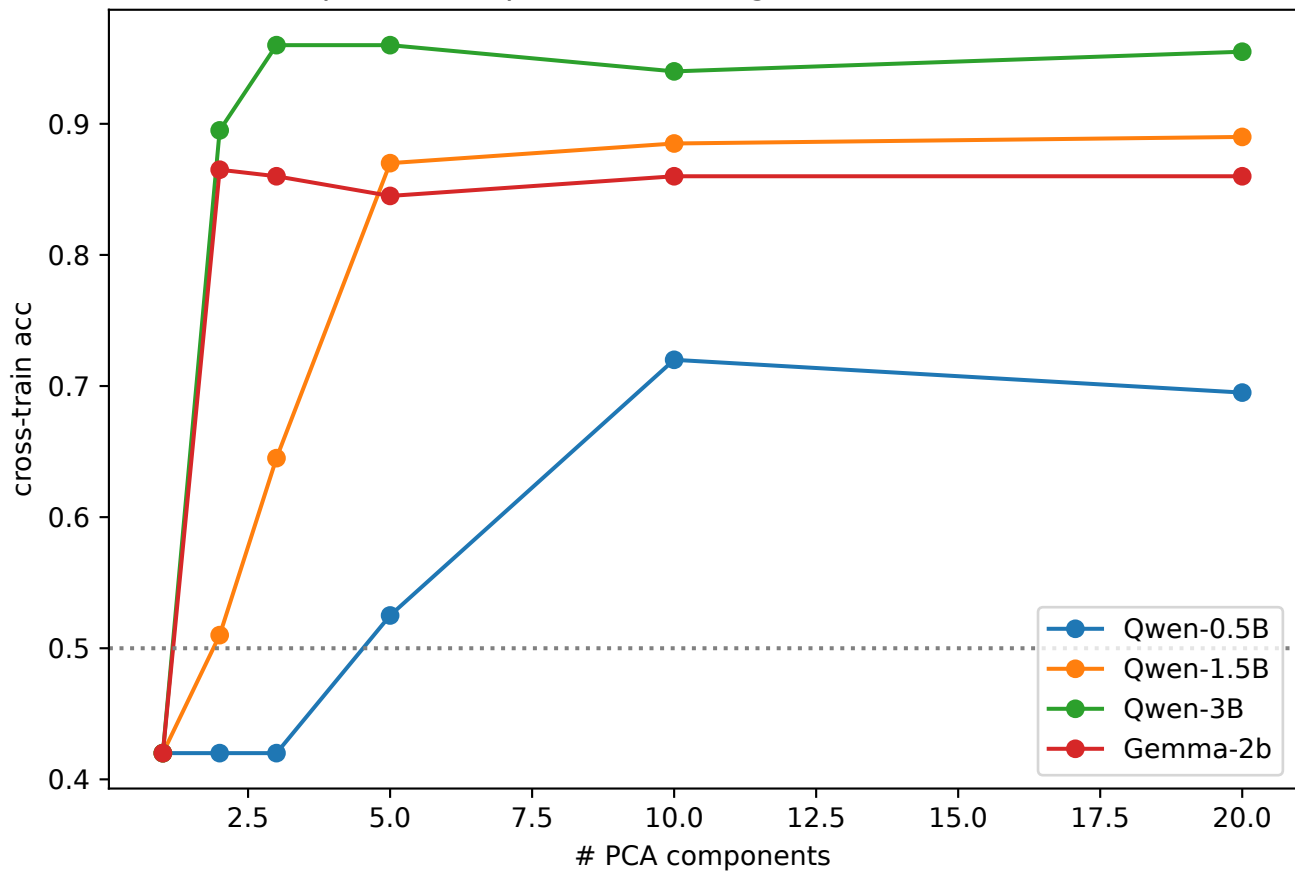
Components required for the signal fall with model scale
