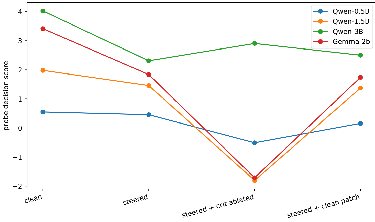
Sufficiency: clean-patch restores the steered score toward clean
