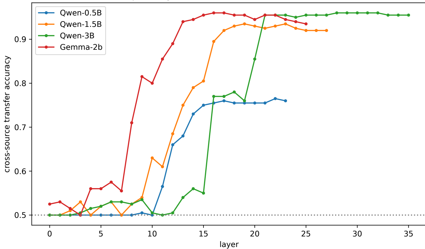
Deception signal transfers across statement sources
