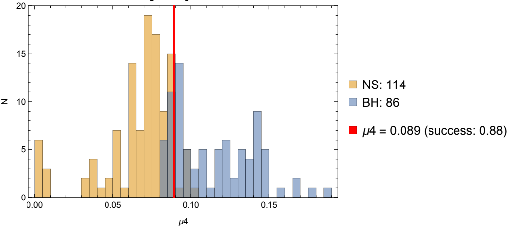
True NS and BH Progen+Engine Data W18-BH2.7-a2.0
