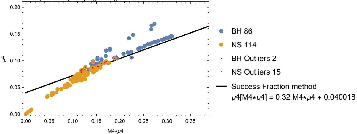
\mu_4 vs M_4*\mu_4 of progen+engine data W18-BH2.7-a2.0
