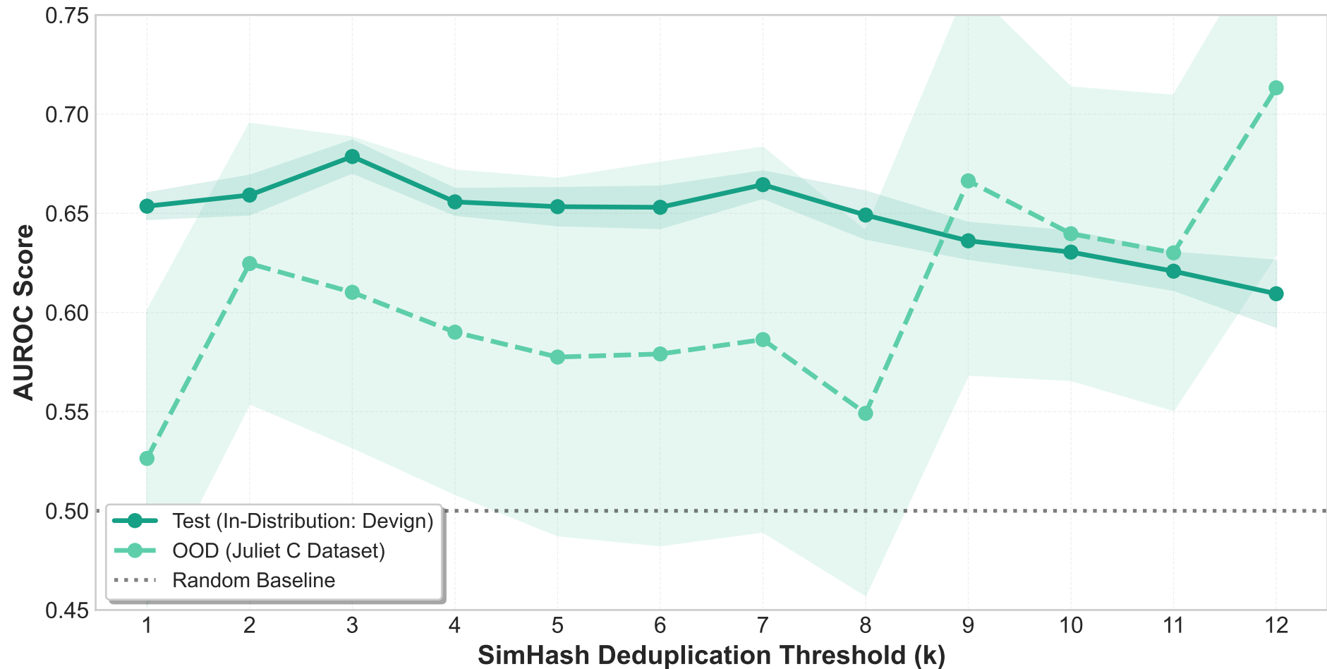
Impact of Deduplication on Model Generalization (Devign Dataset - DeepSeek-6.7B Embeddings)
