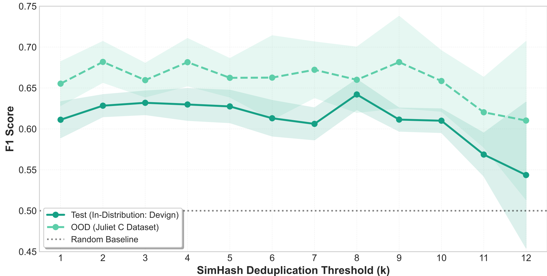
Impact of Deduplication on F1 Score Performance (Devign Dataset - DeepSeek-6.7B Embeddings)
