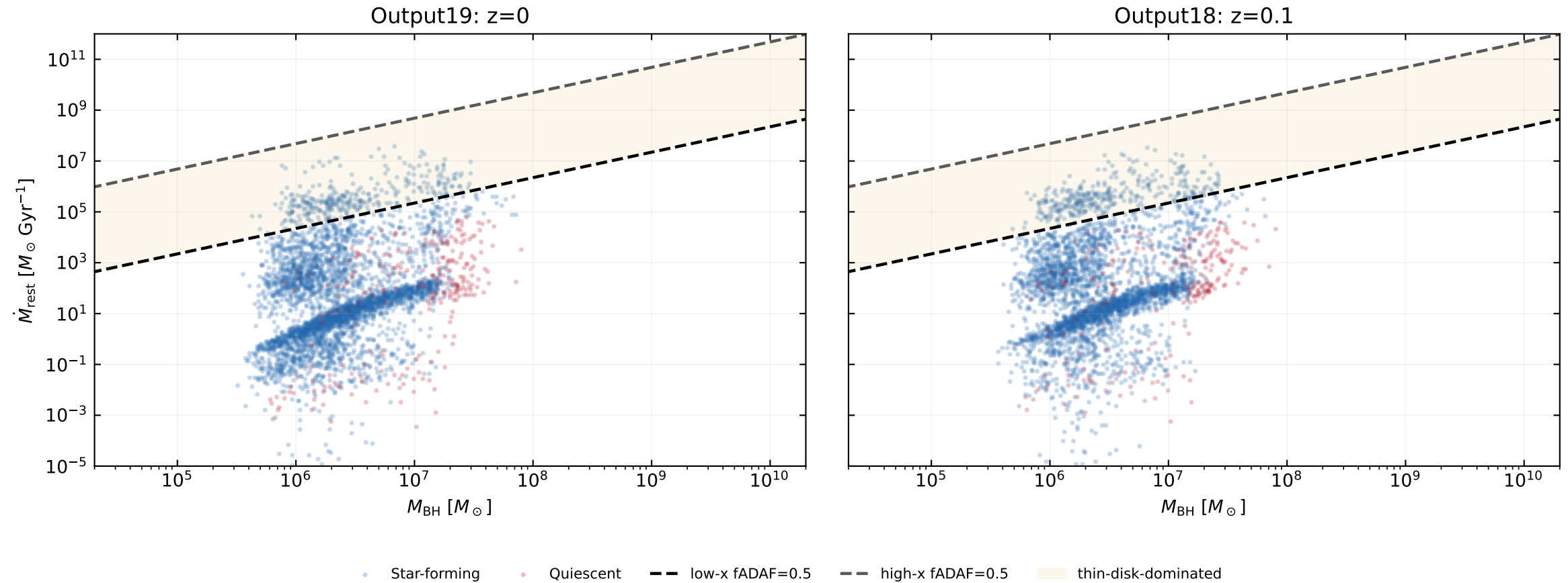
Galacticus accretion states (Paper-II Fig. 5-style); dashed lines are smooth-switch midpoints
