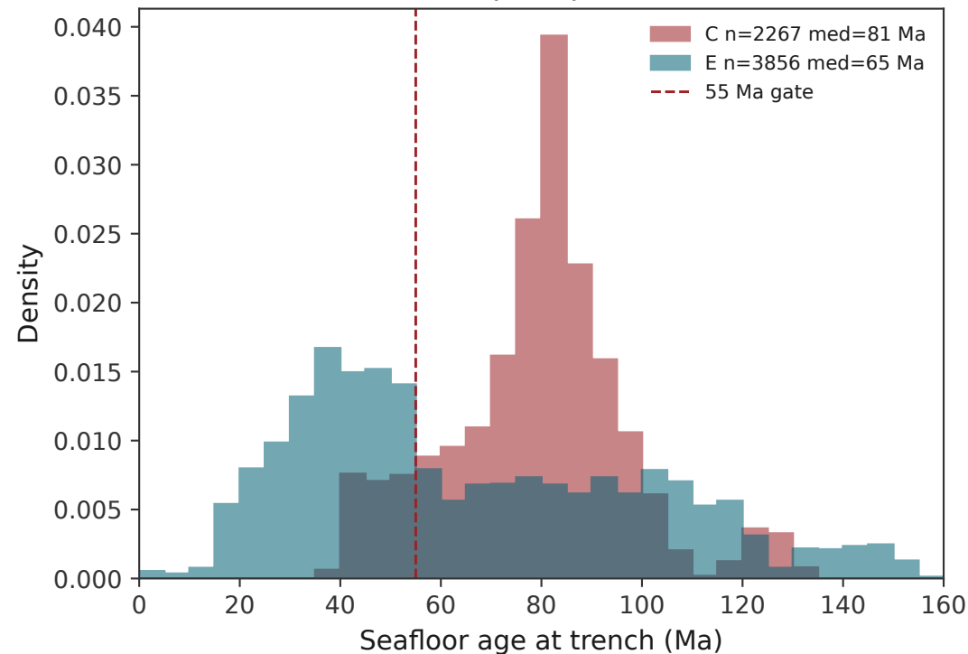
Classified samples, pooled 0-60 Ma
