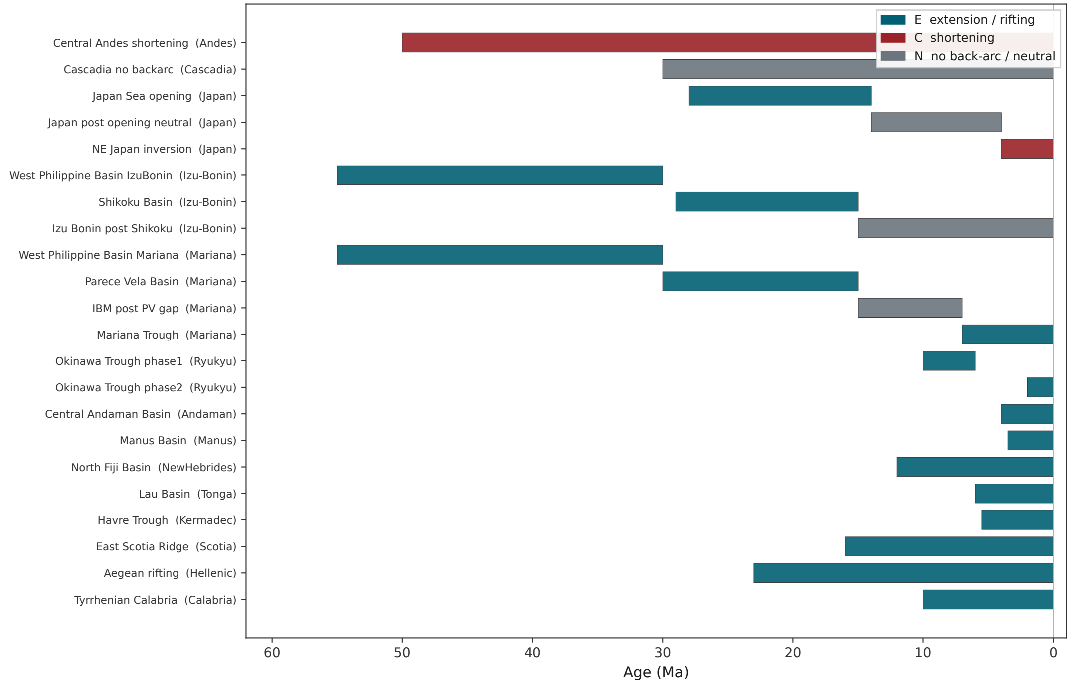
Geological UPS intervals (published ages; not Müller topologies)
