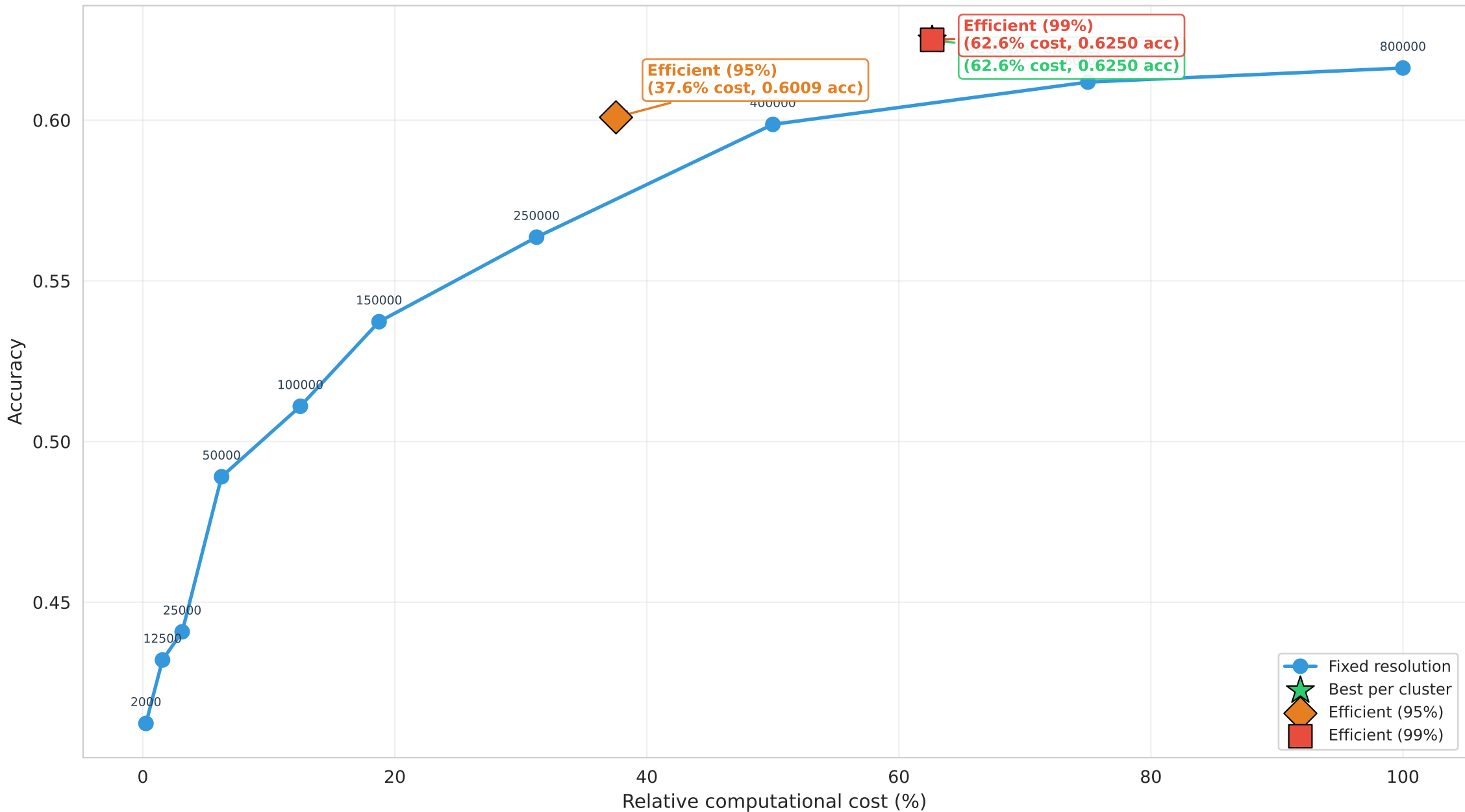
Test set — Accuracy vs. computational cost
