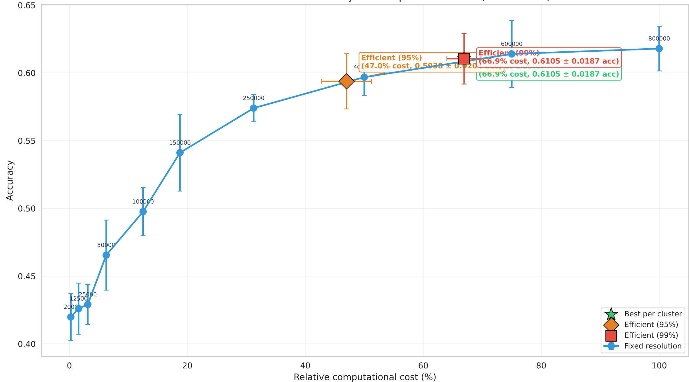
5-fold cross-validation - Accuracy vs. computational cost (mean \pm std)
