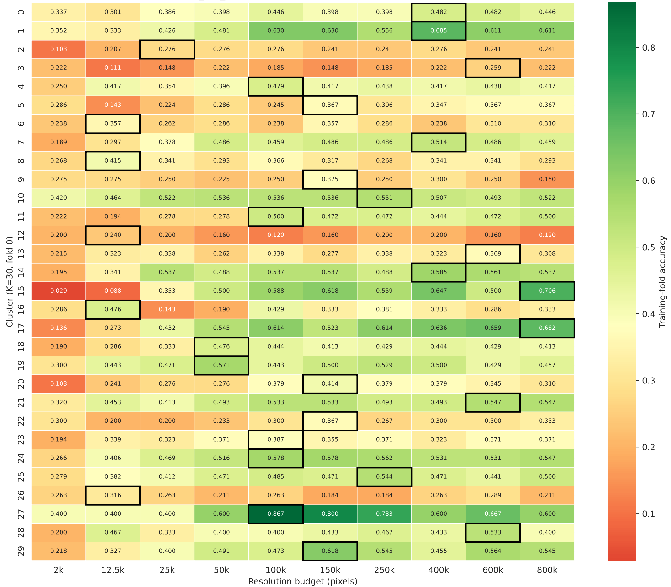
mmmu_pro_standard — per-cluster accuracy by budget
