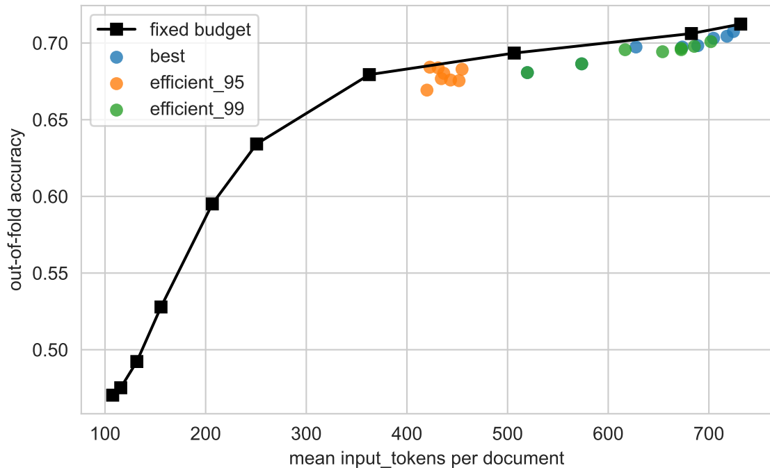
seedbench_2_plus
