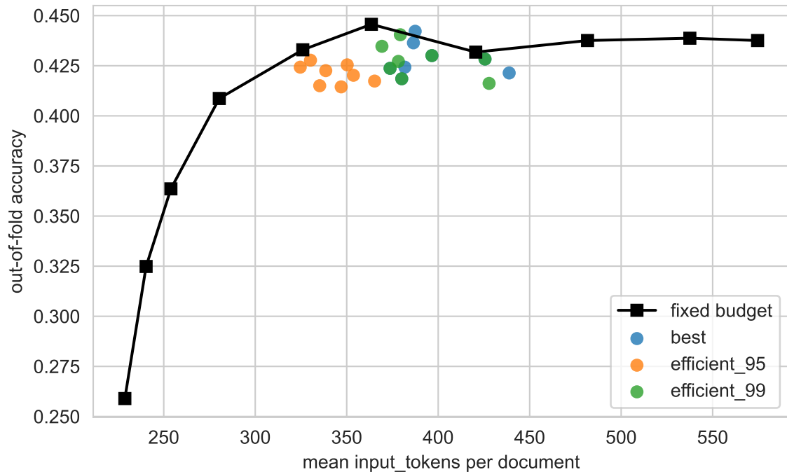
mmmu_pro_standard
