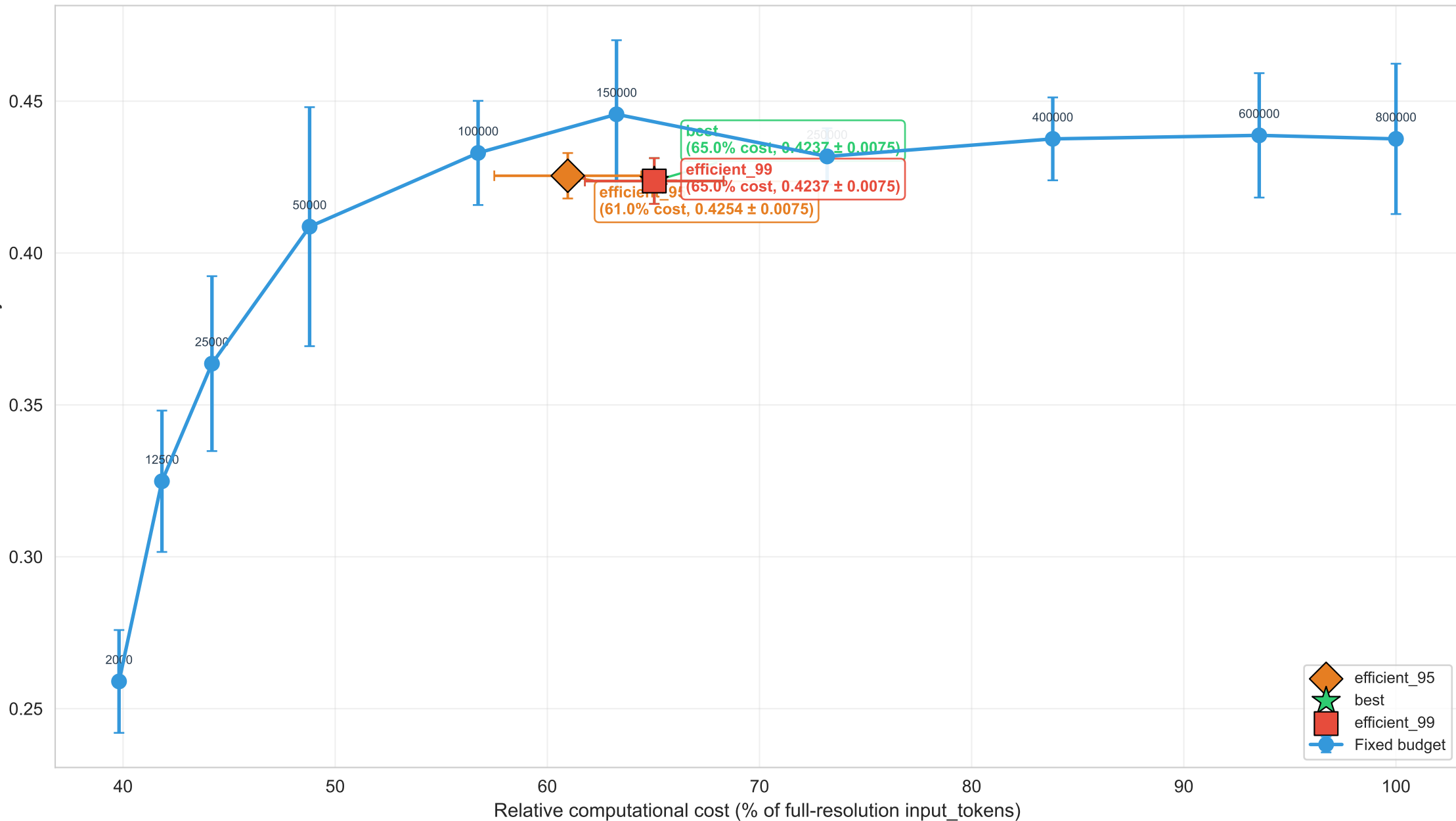
mmmu_pro_standard — 5-fold CV, K=30: accuracy vs cost (mean \pm std)
