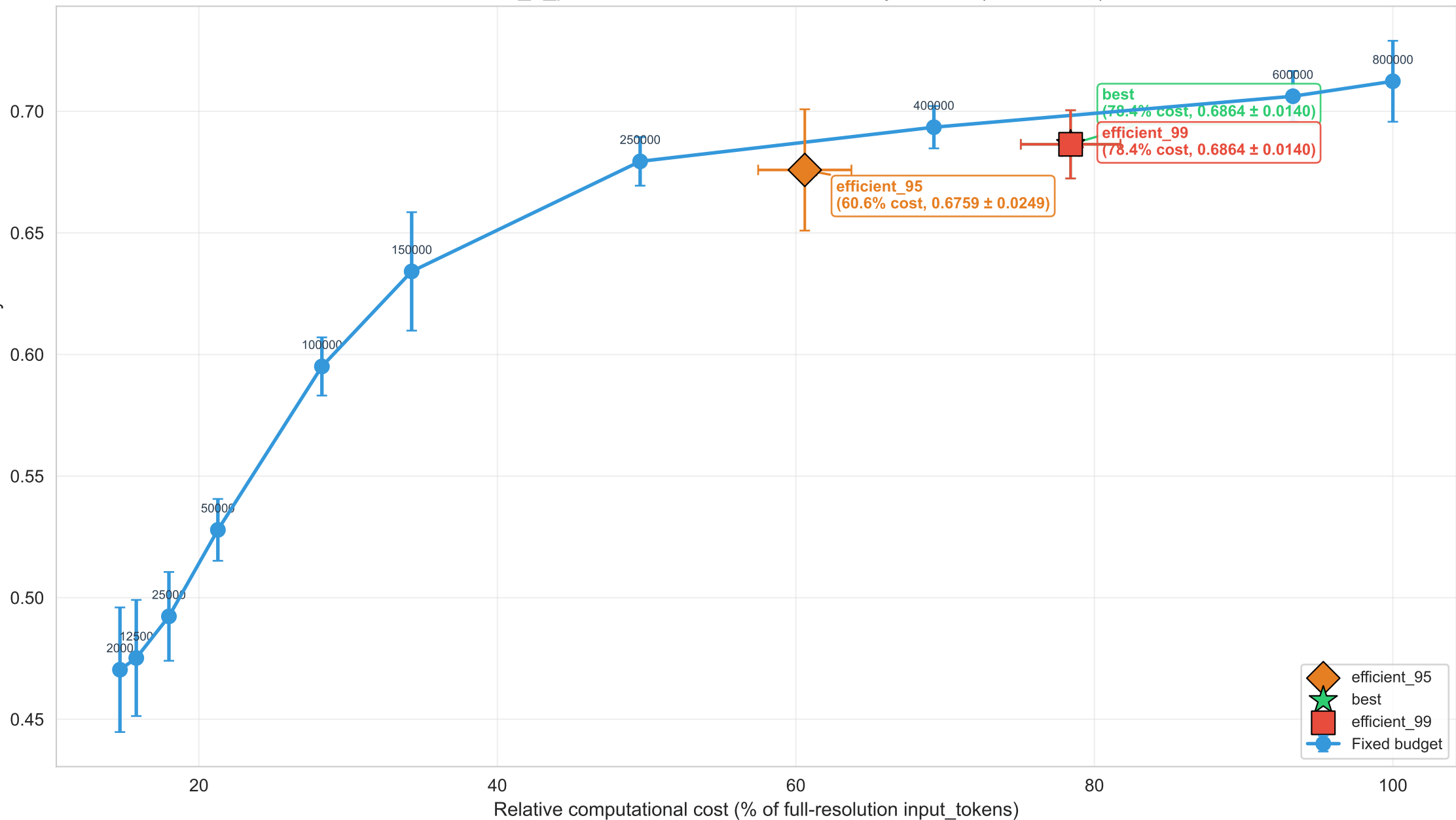
seedbench_2_plus — 5-fold CV, K=30: accuracy vs cost (mean \pm std)
