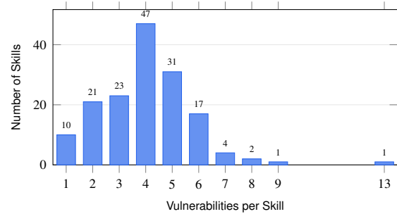
Figure 4: Vulnerability density distribution. The peak at 4 and heavy right tail (80.3% with \geq 3 , up to a single 13-vulnerability outlier) indicate systematic technique layering.
