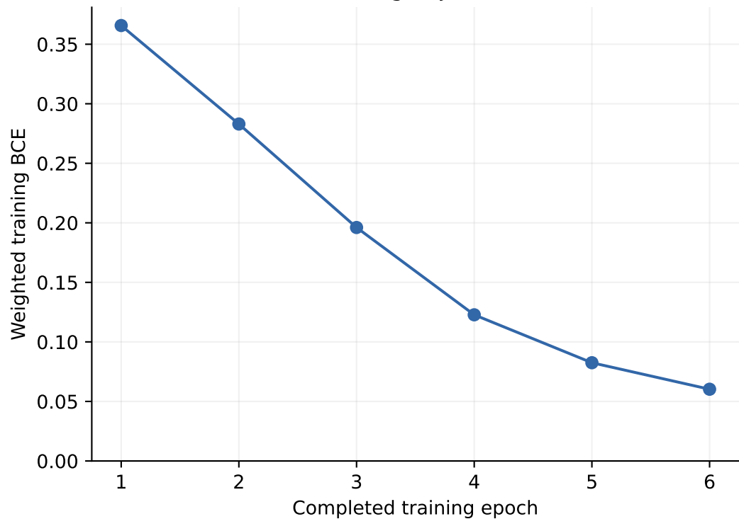
Training objective
