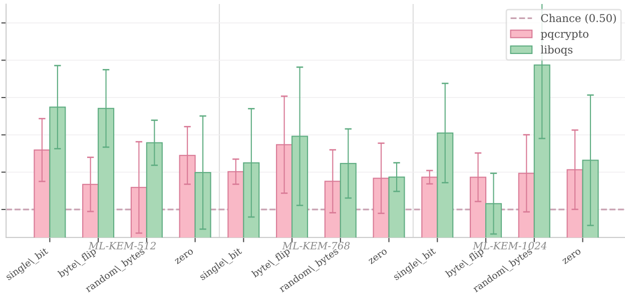
Real-scenario Best-model Accuracy: pqcrypto vs. liboqs
