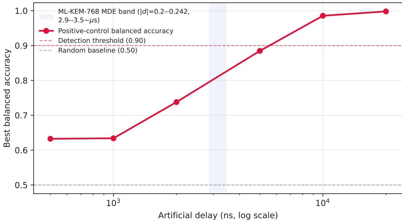
Delay sweep with analytical minimum-detectable-effect band
