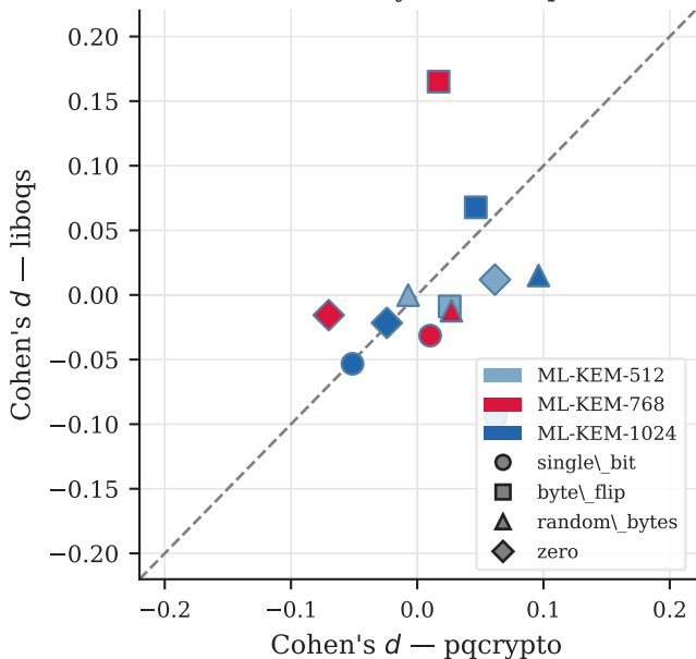
Effect Size Consistency across Implementations
