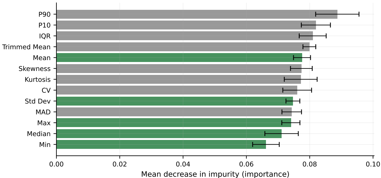
Random Forest feature importance — real scenario (mean \pm std over 8 CV folds)
