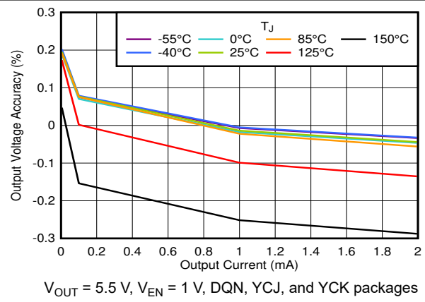
Figure 5-18. Output Voltage Accuracy vs I_{OUT}
