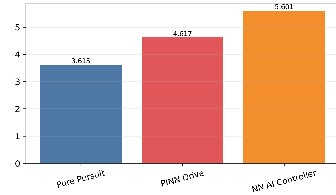
Mean Overshoot Y [%]
