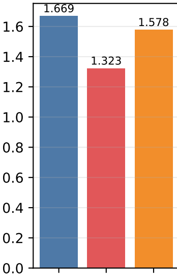
Mean Settling Time Y [s]
