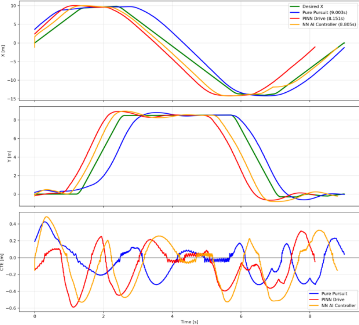
Tracking Comparison | Lap 2 | X / Y / CTE vs Time
