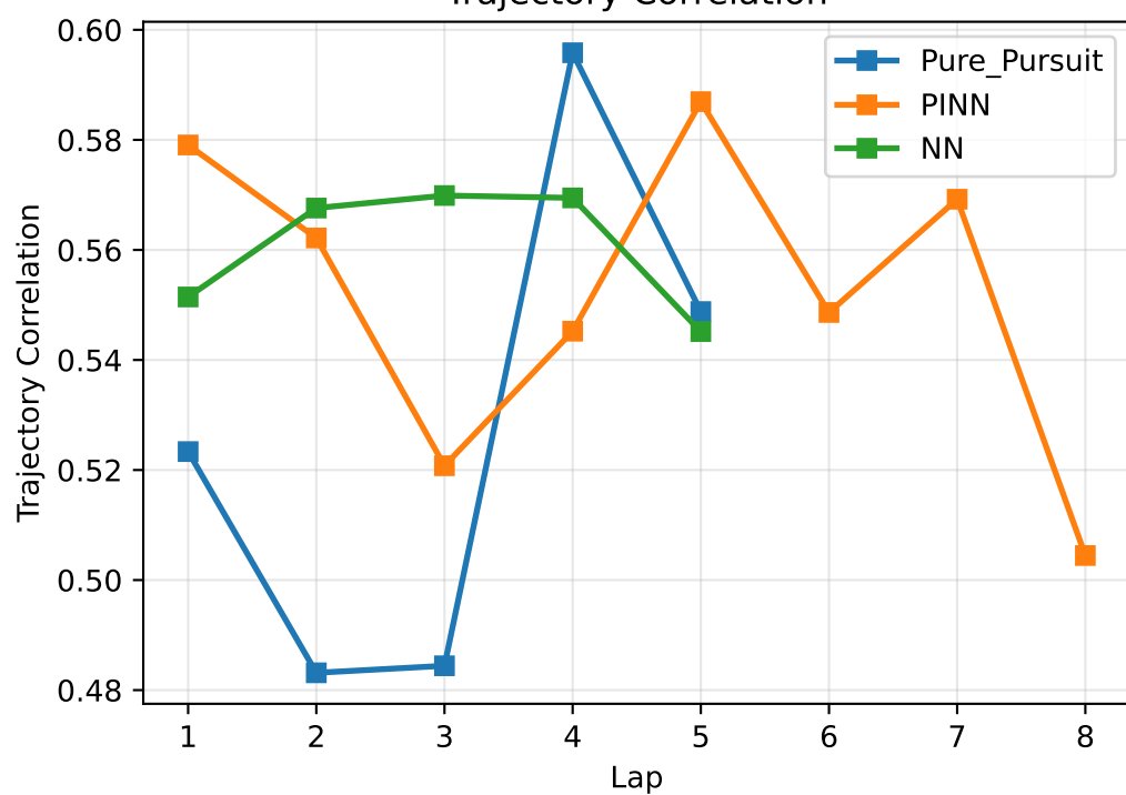
Trajectory Correlation
