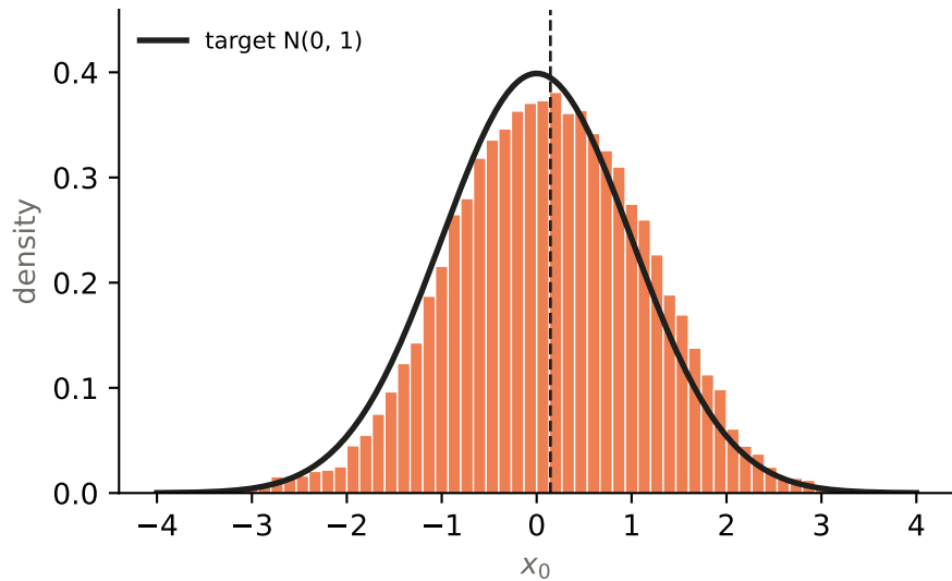
before (v0.8 calibration) mean = +0.145, KS p = 0.0046
