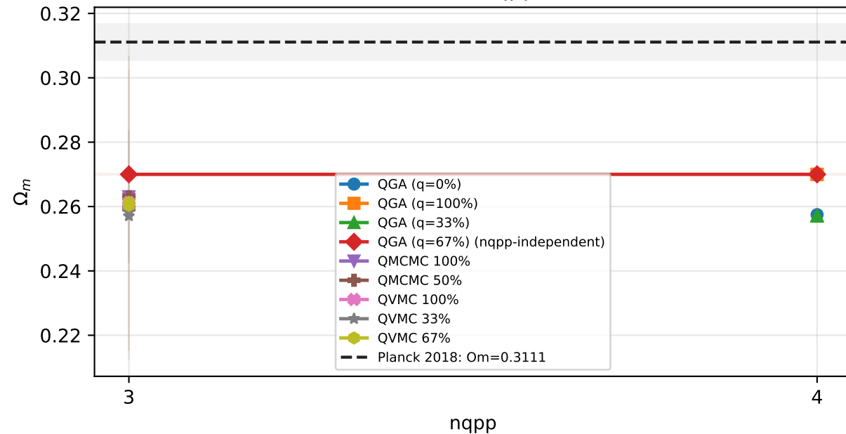
\Omega_m vs nqpp
