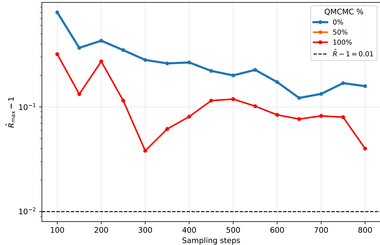
QMCMC convergence along the quantumness ladder (total steps = 800)
