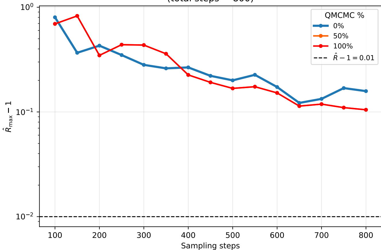
QMCMC convergence along the quantumness ladder (total steps = 800)
