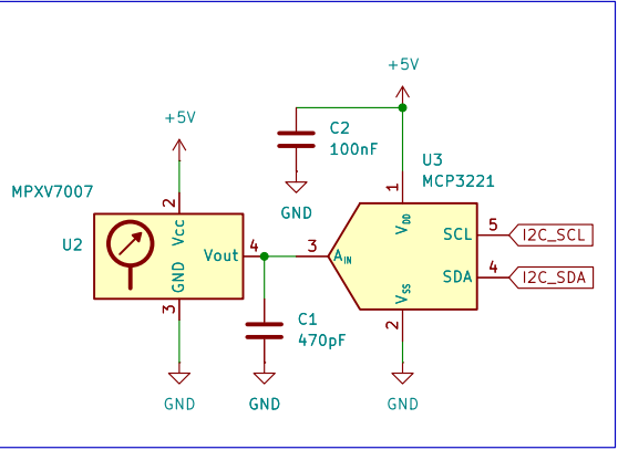
Differential pressure sensor
