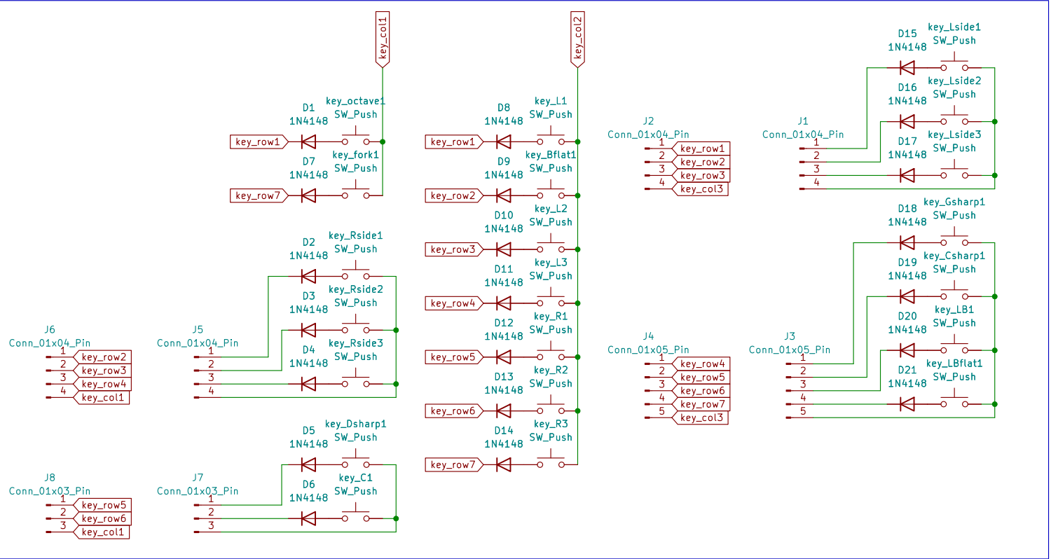
Key matrix
