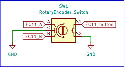
Rotary encoder
